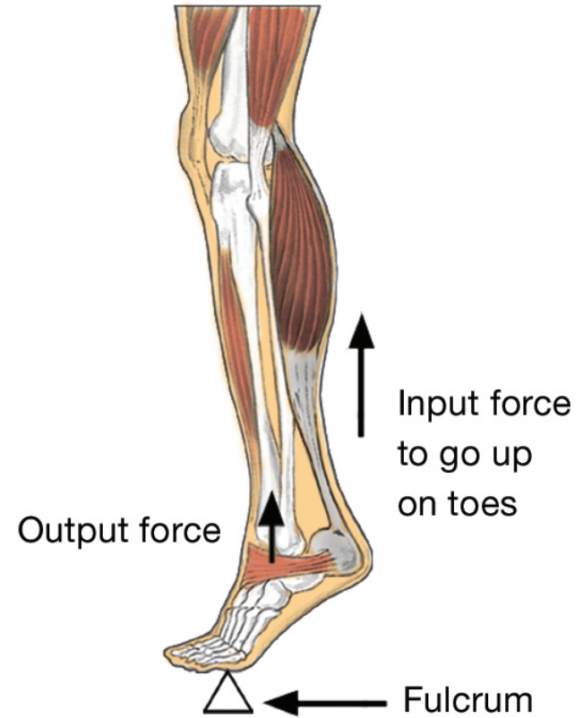
The foot: a second-class lever
