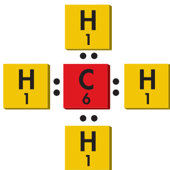
CH 4 Methane
