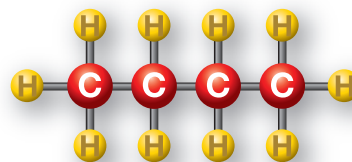
Butane C_4H_{10}
