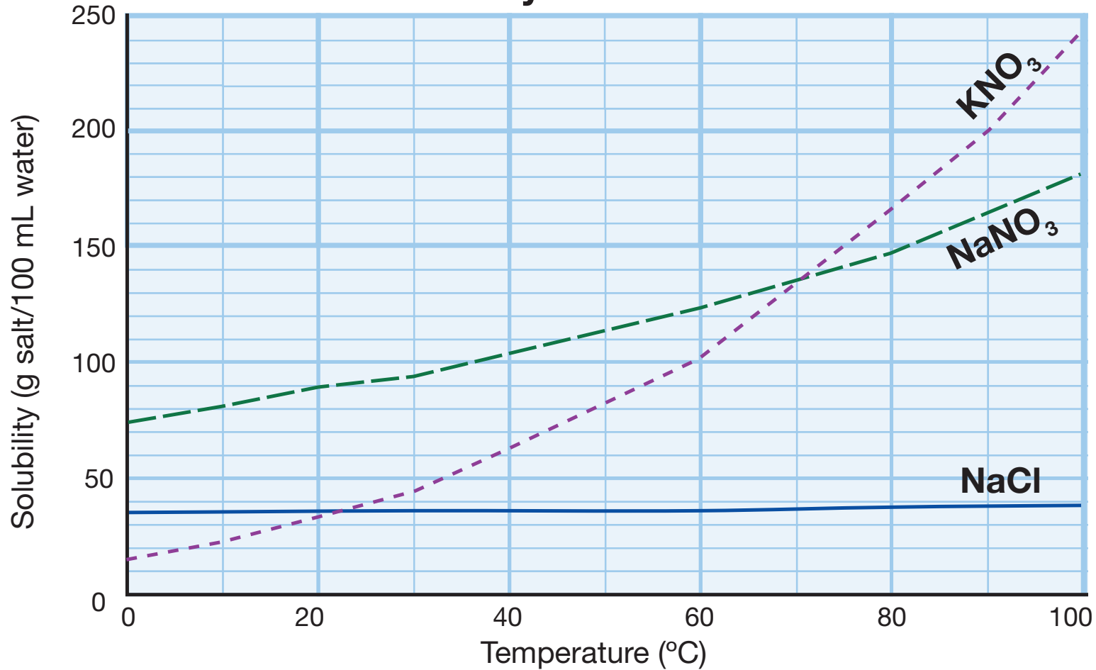
Solubility Curve for Salts
