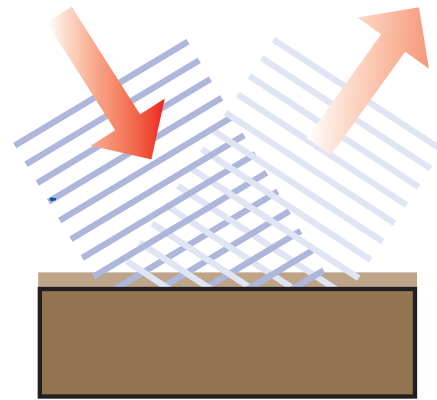
Absorption
