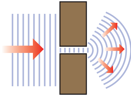
Diffraction
