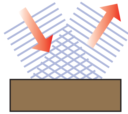
Reflection
