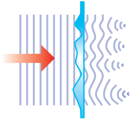
Refraction
