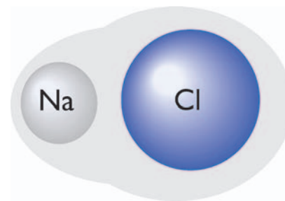
Figure 19.6: Sodium and chlorine form an ionic bond to make sodium chloride (table salt).
